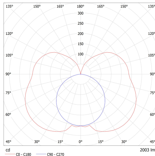
Luminaire: Lucis I3.L4.900.X IZAR III LED Lamps: 1 x LED G6
