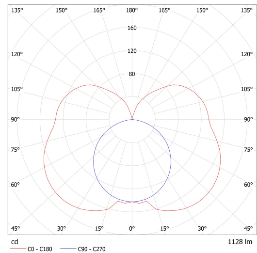
Luminaire: Lucis I3.L3.600.X IZAR III LED Lamps: 1 x LED G6
