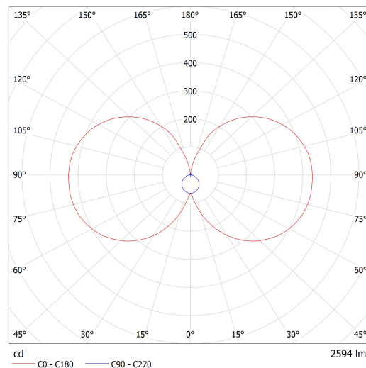
Luminaire: Lucis I2.L4.1200.X IZAR II LED Lamps: 1 x LED G6
