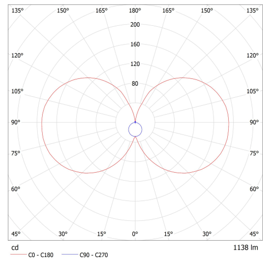
Luminaire: Lucis I2.L4.600.X IZAR II LED Lamps: 1 x LED G6
