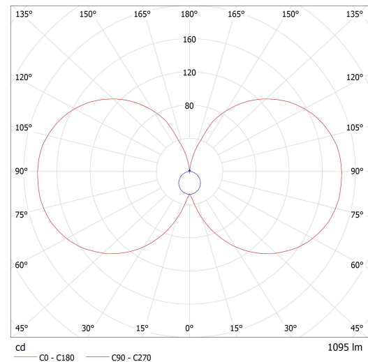
Lucis I2.L3.600.X IZAR II LED / LDC (Polar)
