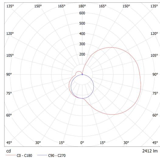
Lucis I1.L4.1200.X IZAR I LED / LDC (Polar)
