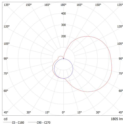
Luminaire: Lucis I1.L4.900.X IZAR I LED Lamps: 1 x LED G6
