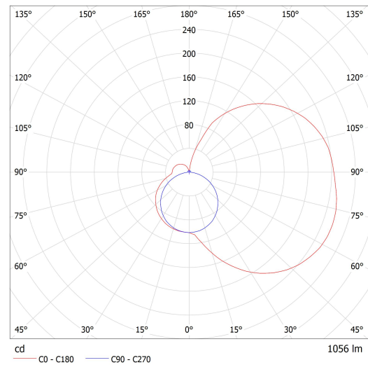
Luminaire: Lucis I1.L4.600.X IZAR I LED Lamps: 1 x LED G6
