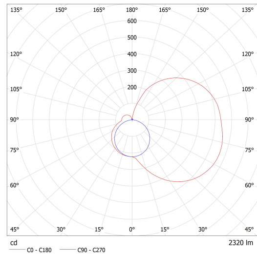
Lucis I1.L3.1200.X IZAR I LED / LDC (Polar)
