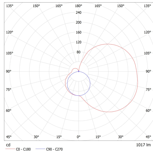
Lucis I1.L3.600.X IZAR I LED / LDC (Polar)
