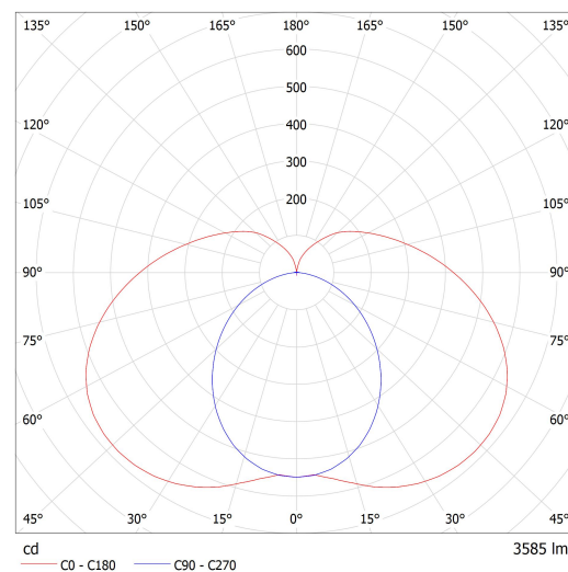
Luminaire: Lucis AU3.L4.1500.X AULA LED Lamps: 1 x LED G6
