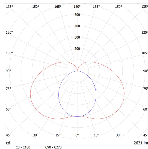
Luminaire: Lucis AU3.L3.1200.X AULA LED Lamps: 1 x LED G6
