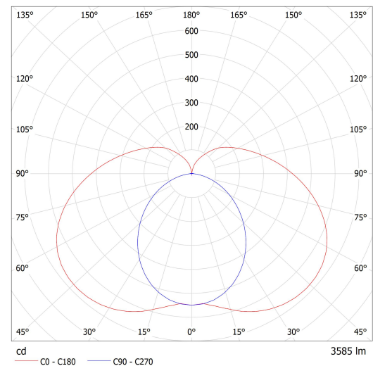
Luminaire: Lucis AU1.L4.1500.X AULA LED Lamps: 1 x LED G6
