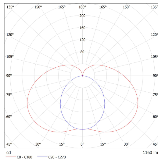
Luminaire: Lucis AU1.L3.600.X AULA LED Lamps: 1 x LED G6
