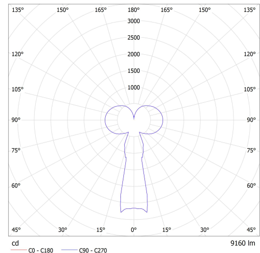
Luminaire: Lucis ZKS.L2A.M620 PA MAIA LED Lamps: 1 x LED G6
