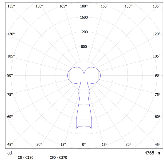
Luminaire: Lucis ZKS.L4A.M500 PA MAIA LED Lamps: 1 x LED G6
