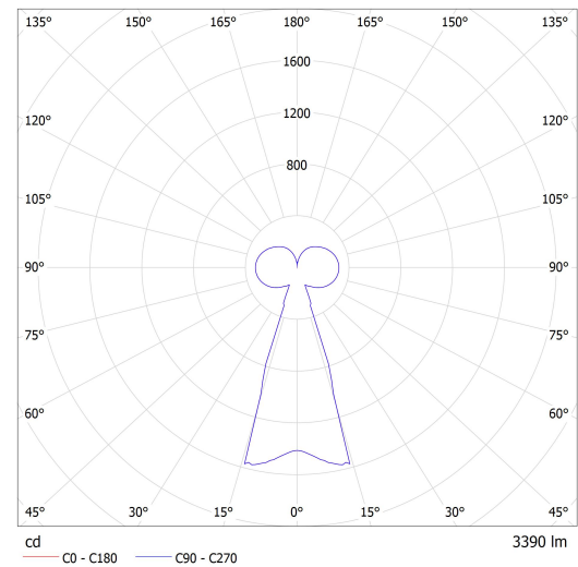
Luminaire: Lucis ZKS.L2A.M320 PA MAIA LED Lamps: 1 x LED G6
