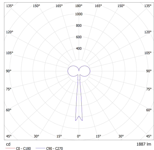
Luminaire: Lucis ZKS.L2A.M580 MAIA LED Lamps: 1 x LED G6
