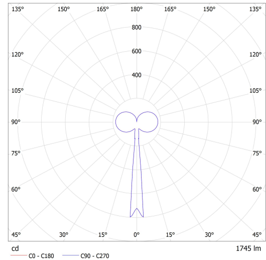
Luminaire: Lucis ZKS.L1A.M580 MAIA LED Lamps: 1 x LED G6
