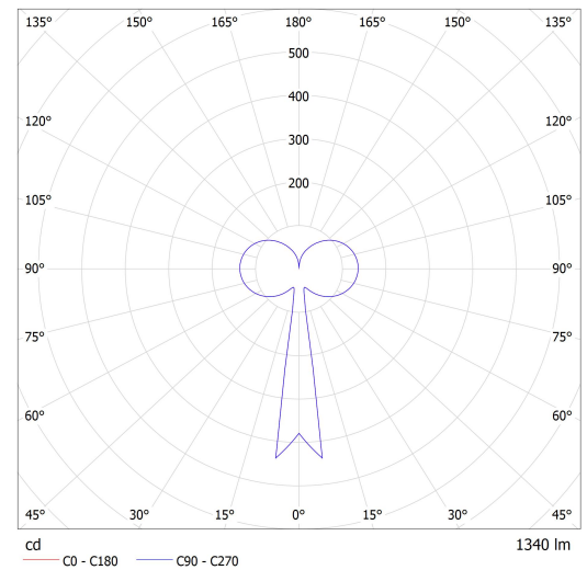
Luminaire: Lucis ZKS.L1A.M380 MAIA LED Lamps: 1 x LED G6
