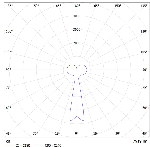
Luminaire: Lucis ZKS.L1A.M620 MAIA LED Lamps: 1 x LED G6
