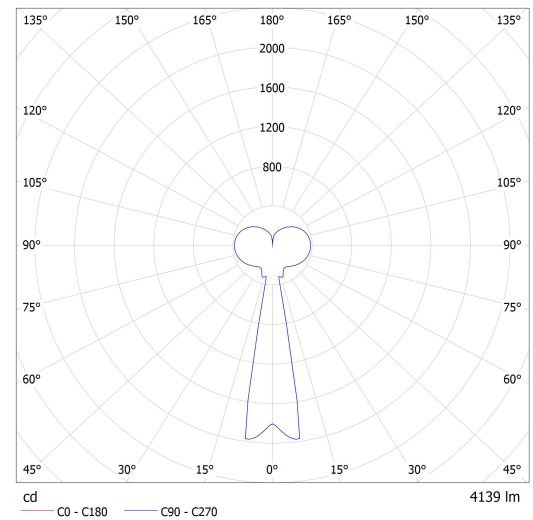
Luminaire: Lucis ZKS.L4A.M500 MAIA LED Lamps: 1 x LED G6
