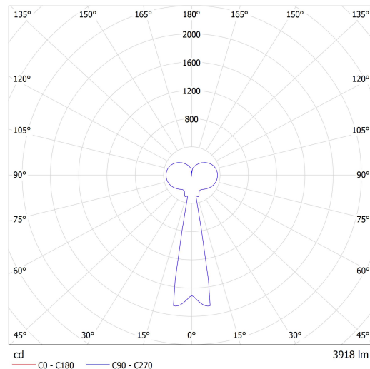
Luminaire: Lucis ZKS.L3A.M500 MAIA LED Lamps: 1 x LED G6
