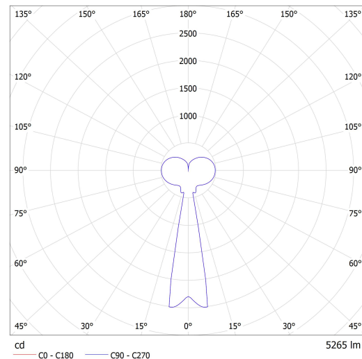
Luminaire: Lucis ZKS.L2A.M500 MAIA LED Lamps: 1 x LED G6
