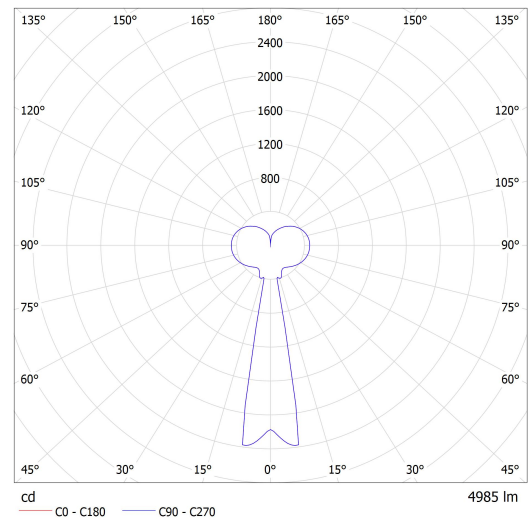
Luminaire: Lucis ZKS.L1A.M500 MAIA LED Lamps: 1 x LED G6
