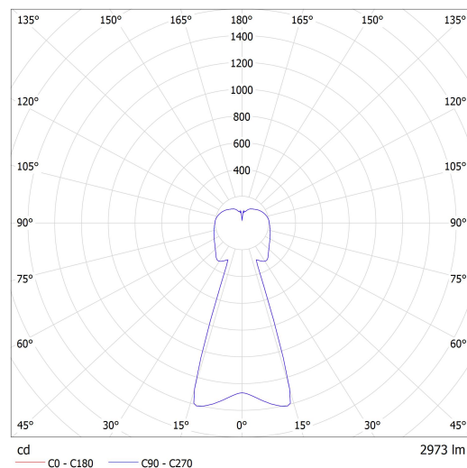
Luminaire: Lucis ZKS.L2A.M320 MAIA LED Lamps: 1 x LED G6
