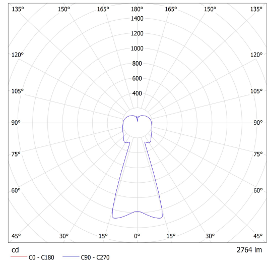
Luminaire: Lucis ZKS.L1A.M320 MAIA LED Lamps: 1 x LED G6
