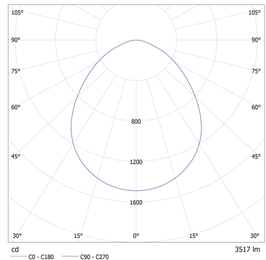
Lucis ZK.K1.J3.X JUNO LED / LDC (Polar)
