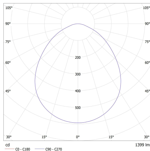
Lucis ZK.K4.J2.X JUNO LED / LDC (Polar)
