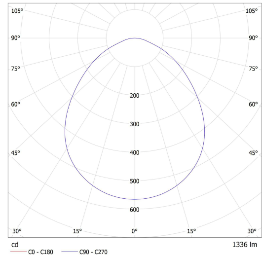
Lucis ZK.K3.J2.X JUNO LED / LDC (Polar)
