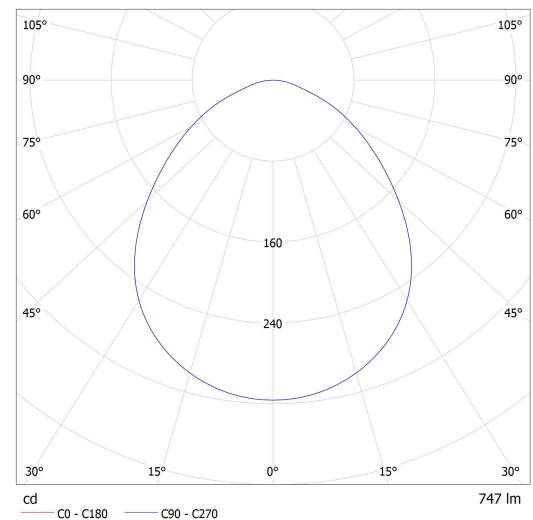
Lucis ZK.K4.J1.X JUNO LED / LDC (Polar)
