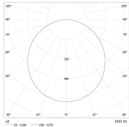
Lucis S7.K1.E220.X ELIOS LED / LDC (Polar)
