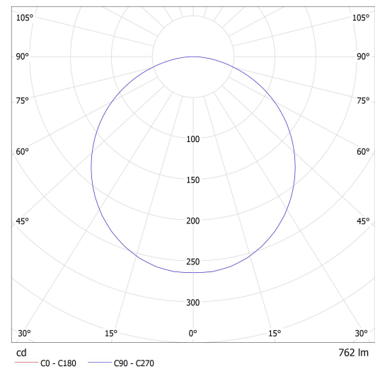
Lucis S7.K4.E120.X ELIOS LED / LDC (Polar)
