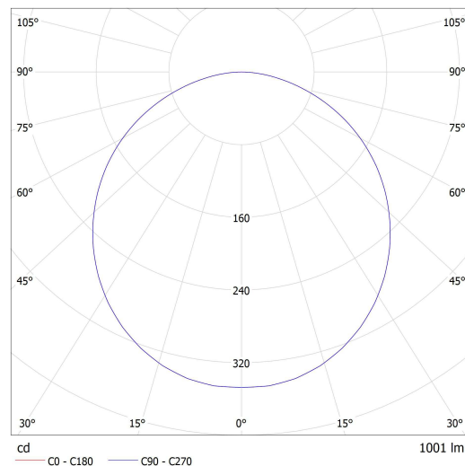
Lucis S7.K1.E120.X ELIOS LED / LDC (Polar)
