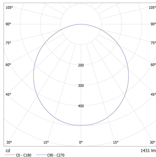
Lucis ZK3.K4.E220.X ELIOS LED / LDC (Polar)
