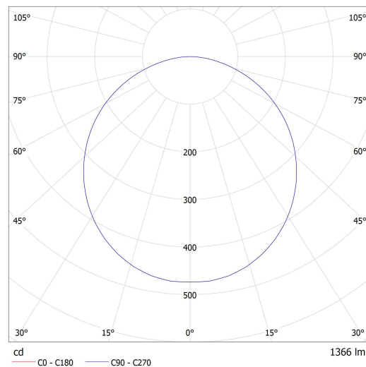
Lucis ZK3.K3.E220.X ELIOS LED / LDC (Polar)
