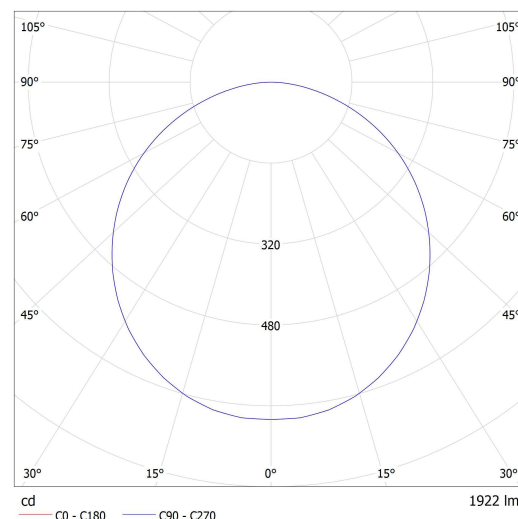
Lucis ZK3.K1.E220.X ELIOS LED / LDC (Polar)
