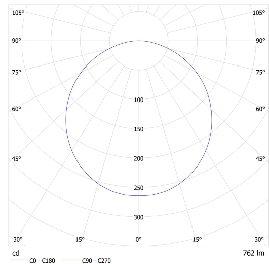
Lucis ZK.K4.E120.X ELIOS LED / LDC (Polar)
