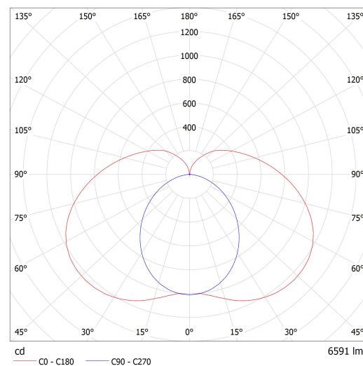
Luminaire: Lucis AU1.L2.1500.X AULA LED Lamps: 1 x LED G6
