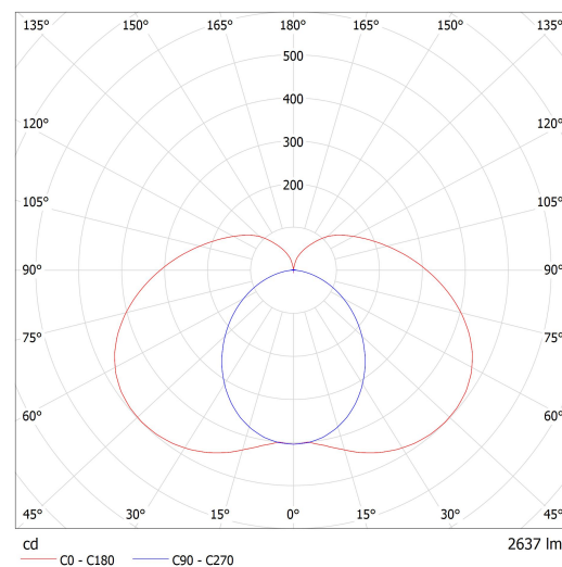
Luminaire: Lucis AU1.L2.600.X AULA LED Lamps: 1 x LED G6
