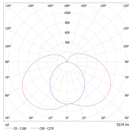
Luminaire: Lucis AU3.L2.1200.X AULA LED Lamps: 1 x LED G6
