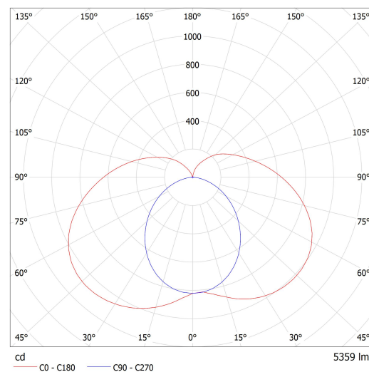
Luminaire: Lucis AU3.L1.1200.X AULA LED Lamps: 1 x LED G6
