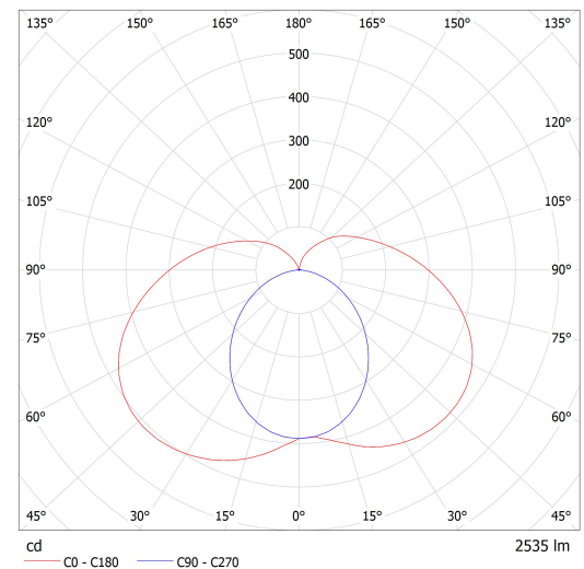
Luminaire: Lucis AU3.L1.600.X AULA LED Lamps: 1 x LED G6
